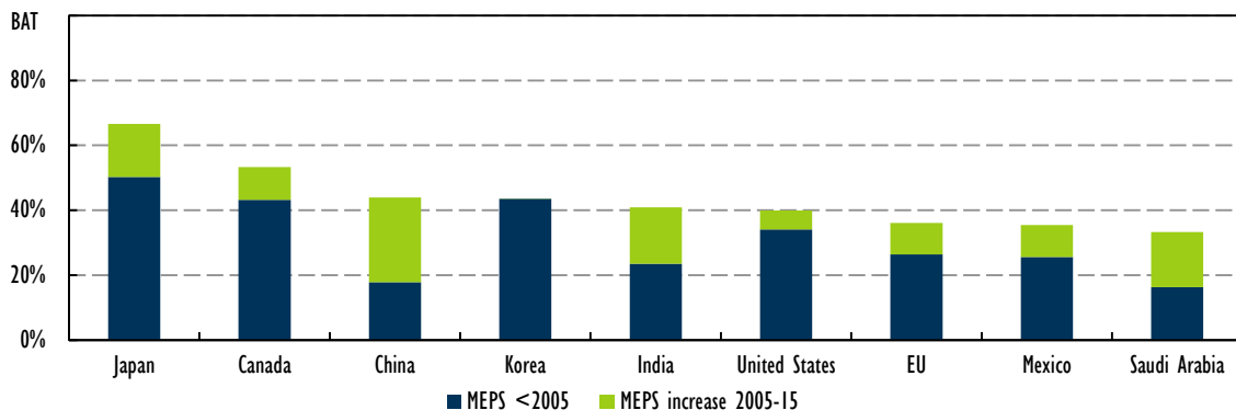
Figure 5.4 Space cooling equipment MEPS for selected countries
